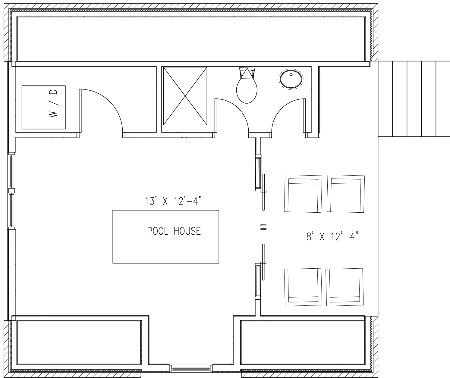
2 DETACHED GARAGE/ POOL HOUSE UPPER LEVEL PLAN 1/4" = 1'-0"
