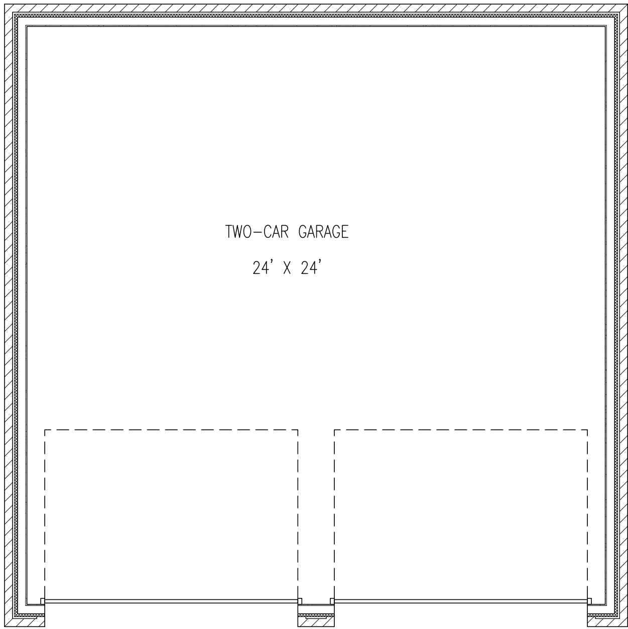
1 DETACHED GARAGE/ POOL HOUSE LOWER LEVEL PLAN 1/4" = 1'-0"
