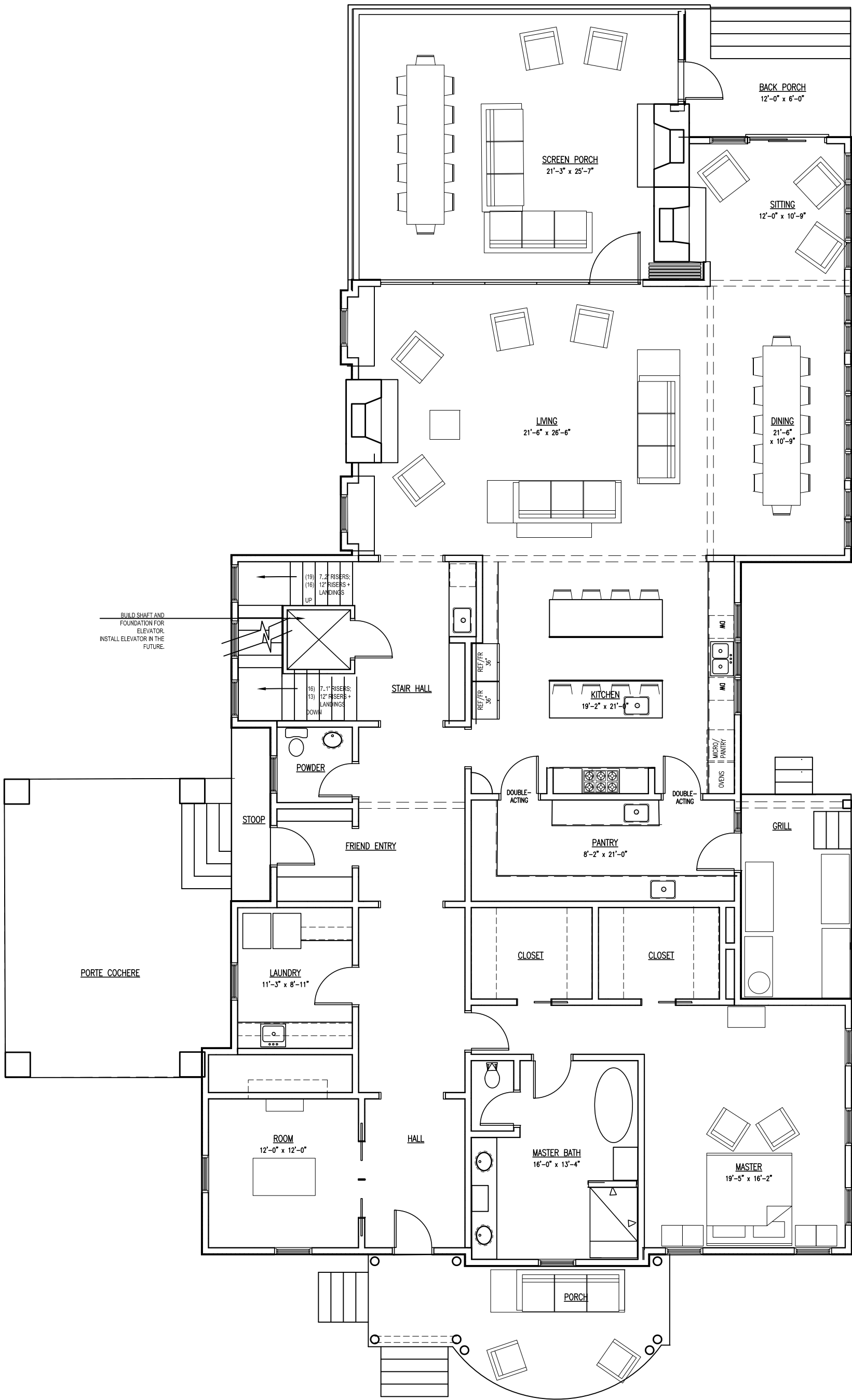
1 First Floor Plan 1/8" = 1'-0"
